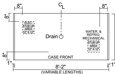
R3 / CR3 Plan View
