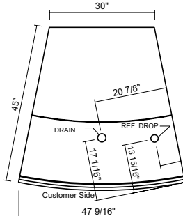
Q3-SS 22.5° Outside Wedge
