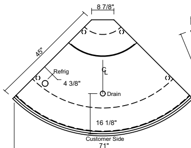
Q3-SS 90° Outside Wedge
