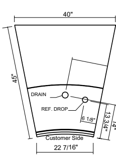
Q3-SS 22.5° Inside Wedge
