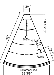
Q3-SS 45° Outside Wedge
