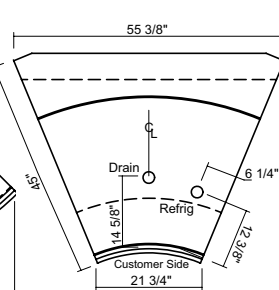
Q3-SS 45° Inside Wedge
